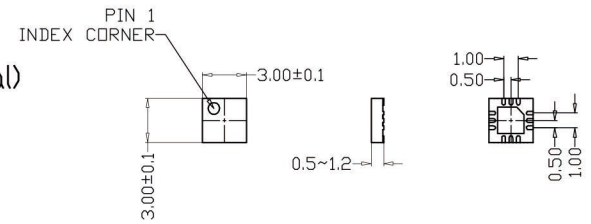
TOP VIEW SIDE VIEW BOTTOM VIEW
