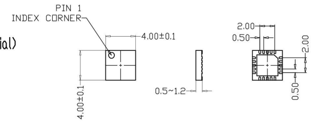
TOP VIEW SIDE VIEW BOTTOM VIEW
