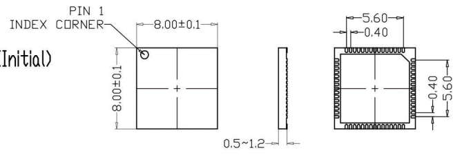
TOP VIEW SIDE VIEW BOTTOM VIEW
