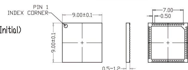
TOP VIEW SIDE VIEW BOTTOM VIEW
