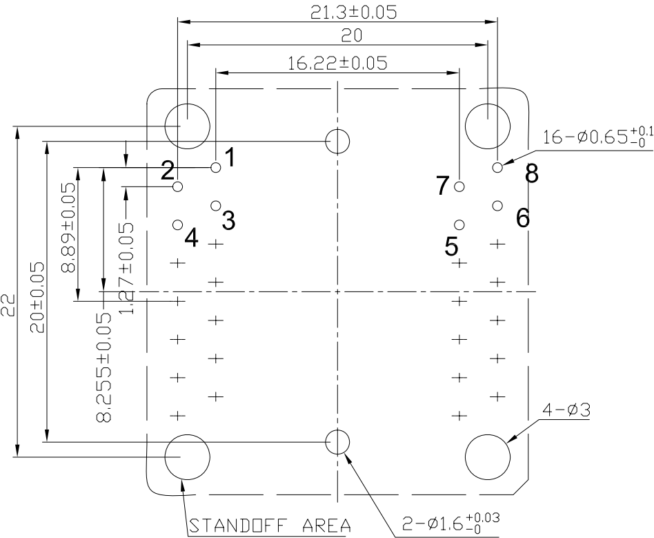
PCB PATTERN (TOP VIEW)
